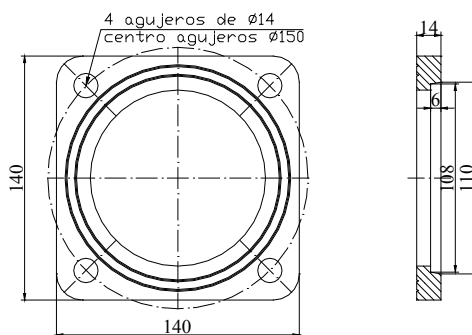
Cast aluminium square flange
