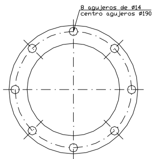
Aluminium tank flange
