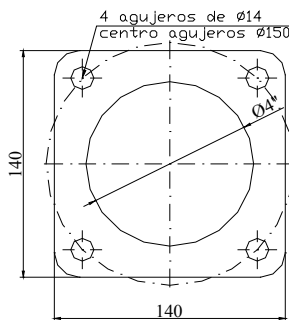
NBR square flange gasket
