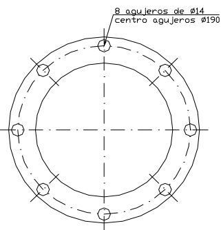
"Vitón" tank flange gasket Art. 940052V
