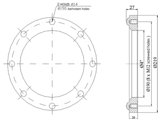
Dimensions / Dimensiones Art.940890FE
